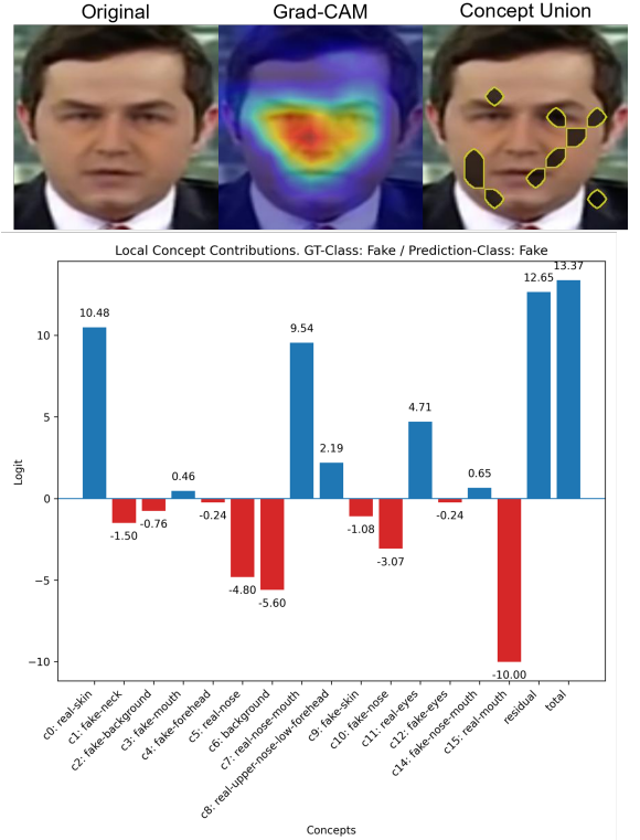
Figure 3. Visualization of the original image, its Grad-CAM heatmap and the union of all Concept Presence Maps (top). Logit decomposition into individual concept contributions and the residual term (bottom)
